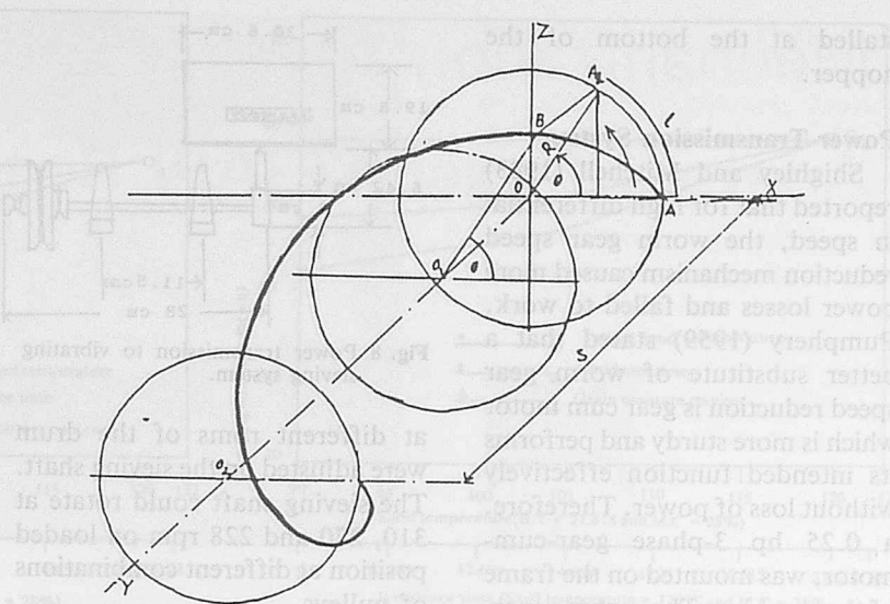
Fig. 6 Determination of coordinates of point (B) on auger convolution helical line.
