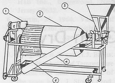
Fig. 1 A view of the continuous dryer (1. gear motor, 2. drying cylinder, 3. grain hopper, 4. augur, 5. sand pan).
