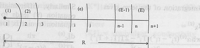
Fig. 1 Discretization of radius of the cylindrical bin into finite element.
