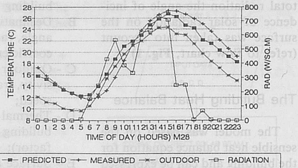
Fig. 5 Predicted and measured temperatures.
