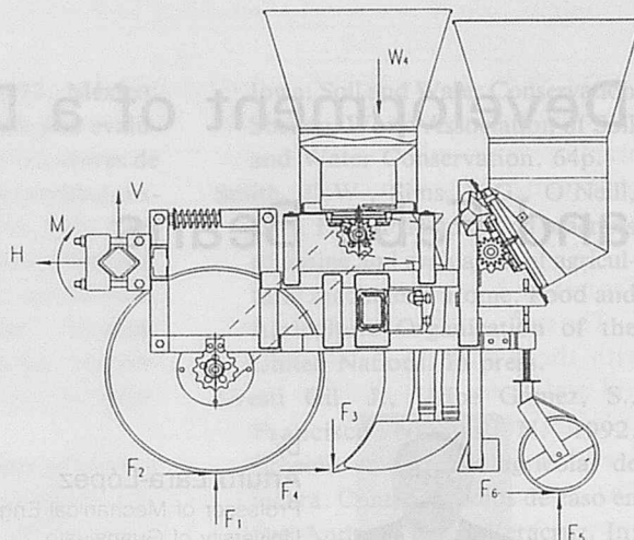
Fig. 3 External forces on planter calculated for normal operation.
