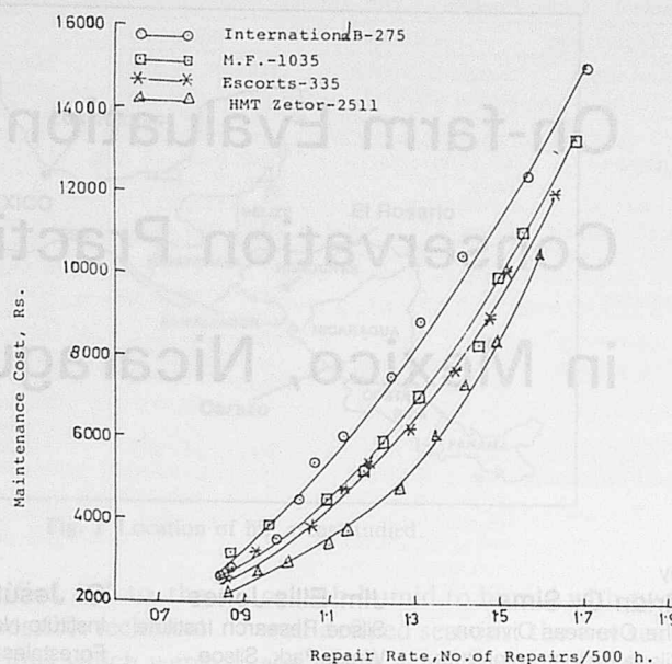
Fig. 2 Relationship between the maintenance cost and repair rate of tractors.
