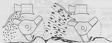
Fig. 6.2 Side views of rotary tiller.
