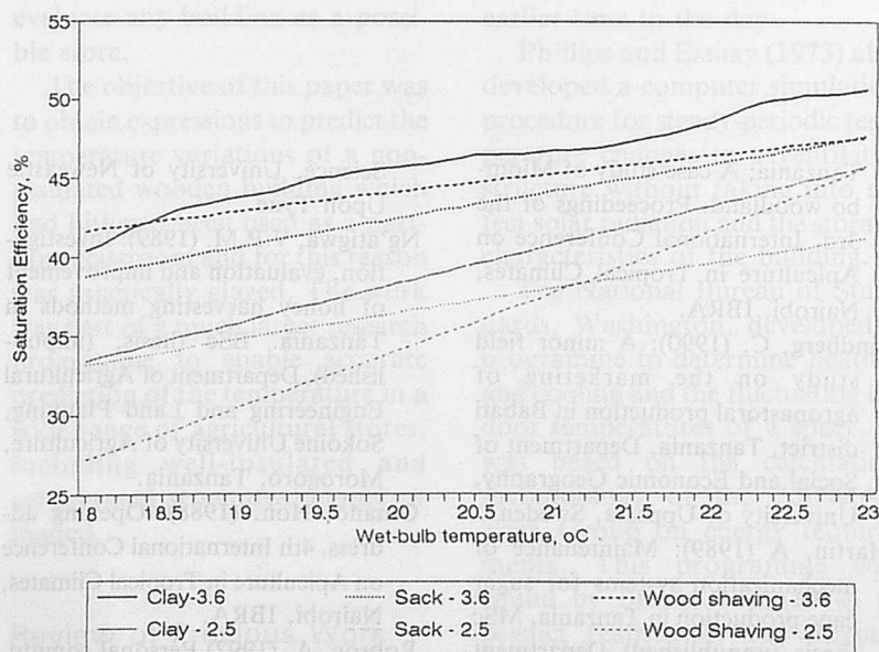
Fig. 3 Saturation efficiency vs wet-bulb temperature.
