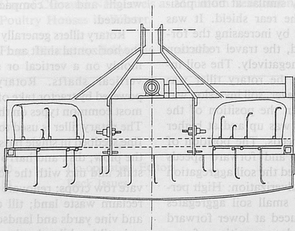
Fig. 6.1 Line diagram of rotary tiller.
