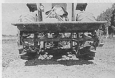
Fig. 2 Rear view of rotary tiller (Shield up).
