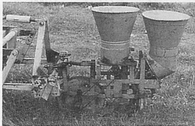
Fig. 4 Planter prototype during test on a field with grass.
