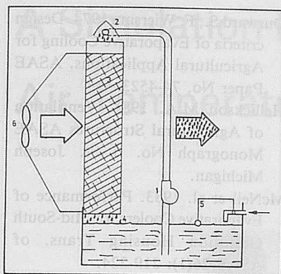
Fig. 1 The evaporative cooling system.
